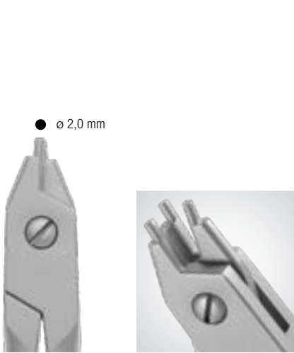
3000/60 ø max 1,4 mm / .055" mm 130 3 prong plier. For hard wires. Round tips prevents any damage of archwire.
